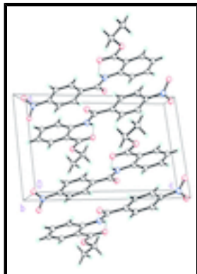
Fig. 2. Packing diagram of the title compound viewed down the b axis. Dashed lined indicate N—H...O intramolecular hydrogen bonding.
